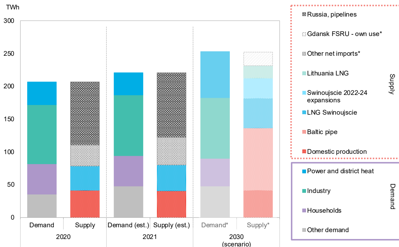
Figure 23: Polish gas supply and gas sources, historic and future scenarios
