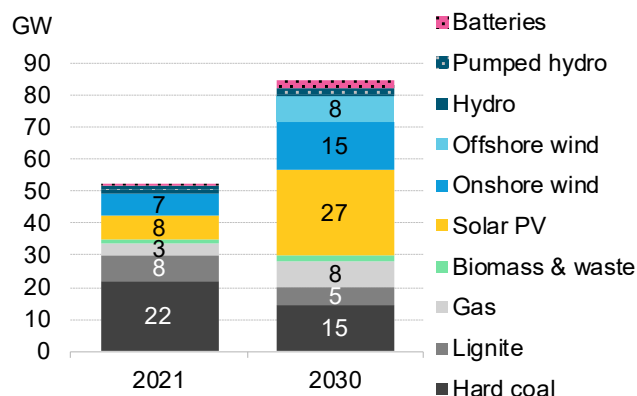
Figure 29: Base-case scenario: installed capacity in 2021 vs. 2030
