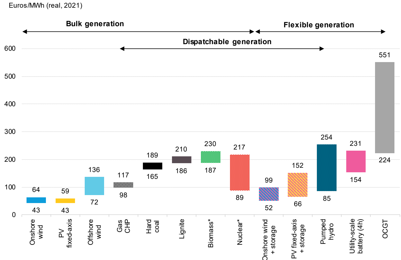
Figure 11: Poland/Germany 2022 levelized cost of electricity ranges per technology
