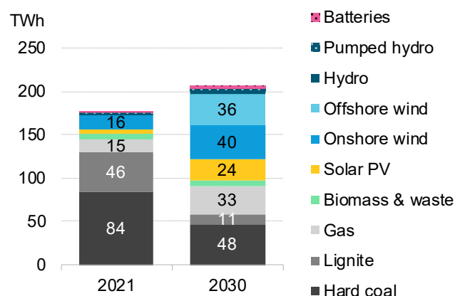
Figure 32: High Gas/Low CO2 Prices Scenario: generation in 2021 vs. 2030
